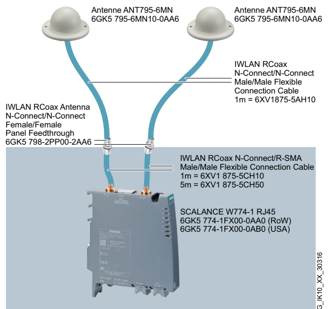
Control cabinet
