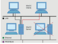
WinCC/Redundancy
